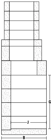
SIDE ELEVATION
