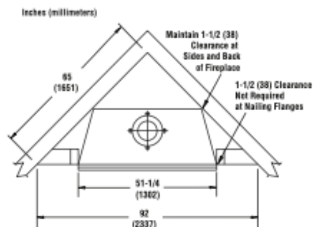
Corner Framing Dimensions
