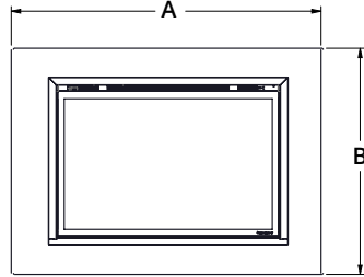
4-Sided Faceplate
