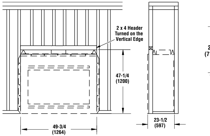
Parallel Framing Dimensions
