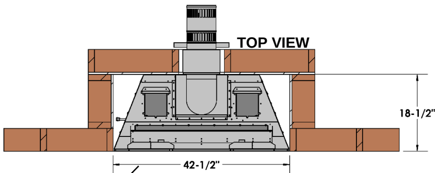
Fig.1 Framing for Horizontal Vent Termination (See Installation of Side Wall Venting Section)
