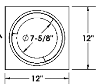
ZDVAIS or Z7AIS24 Attic Insulation Shield
