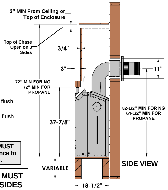
Fig.1 Framing for Horizontal Vent Termination (See Installation of Side Wall Venting Section )
